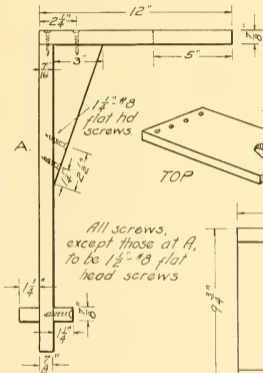
TYPE OF SUPPORT FOR USE IN BENCH VISE, FIG. A
